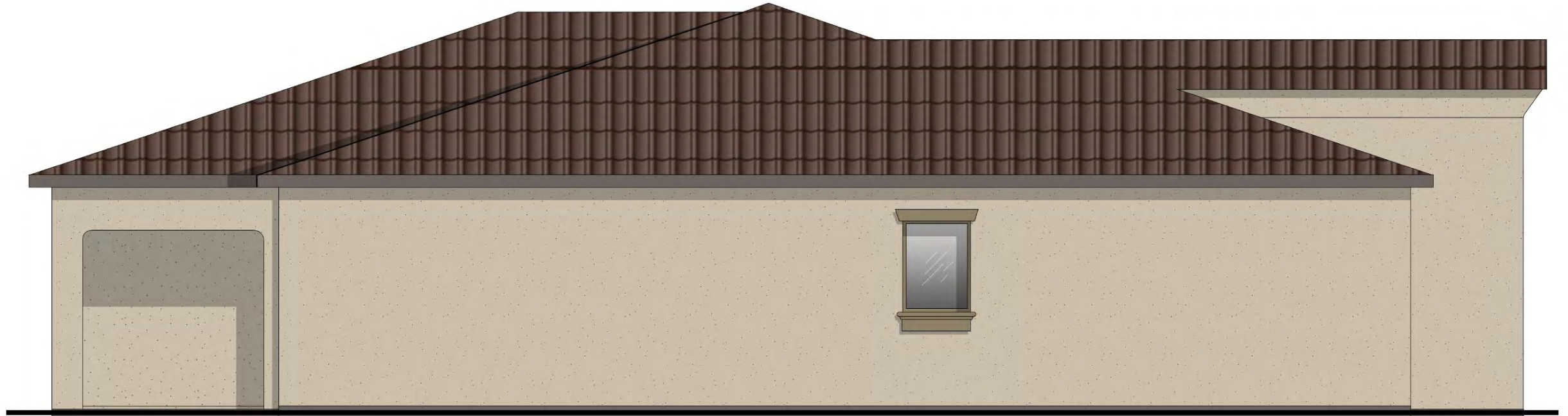
SIDE ELEVATION "A" - SPANISH © HARVEST
