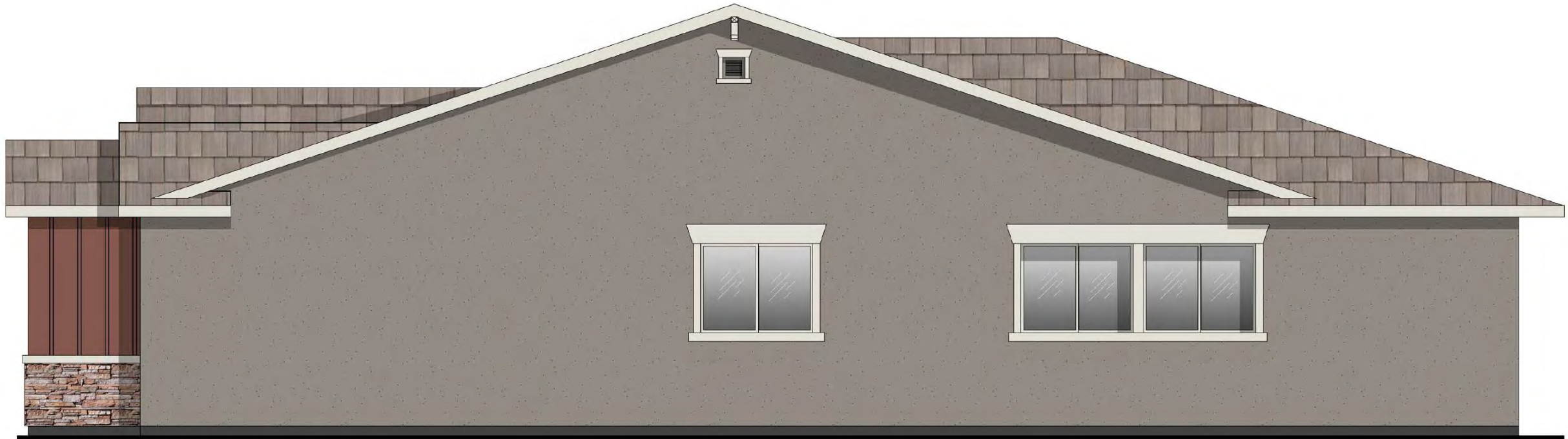
SIDE ELEVATION "B" - CRAFTSMAN @ HARVEST
