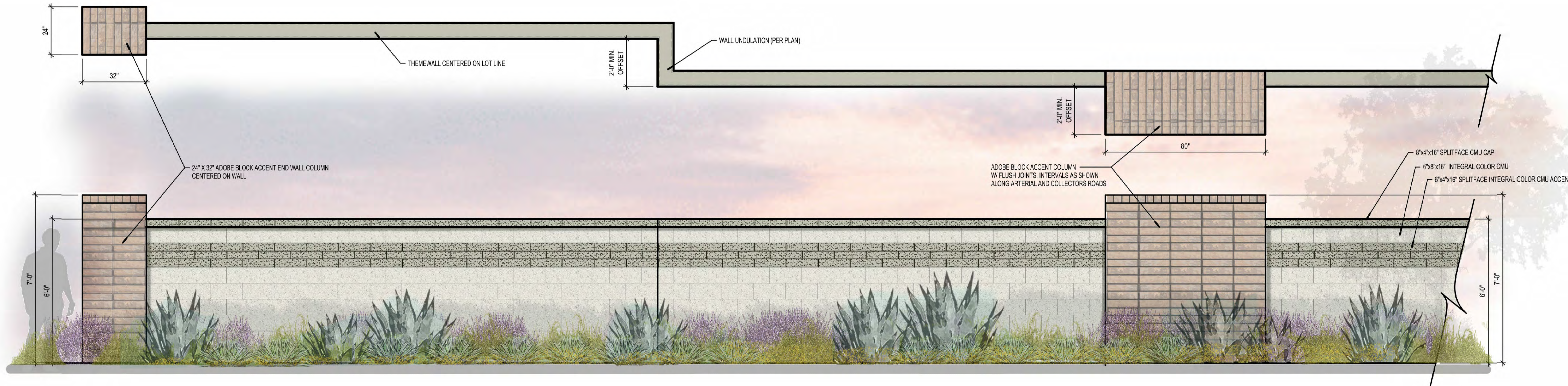
TYPICAL THEME-WALL
