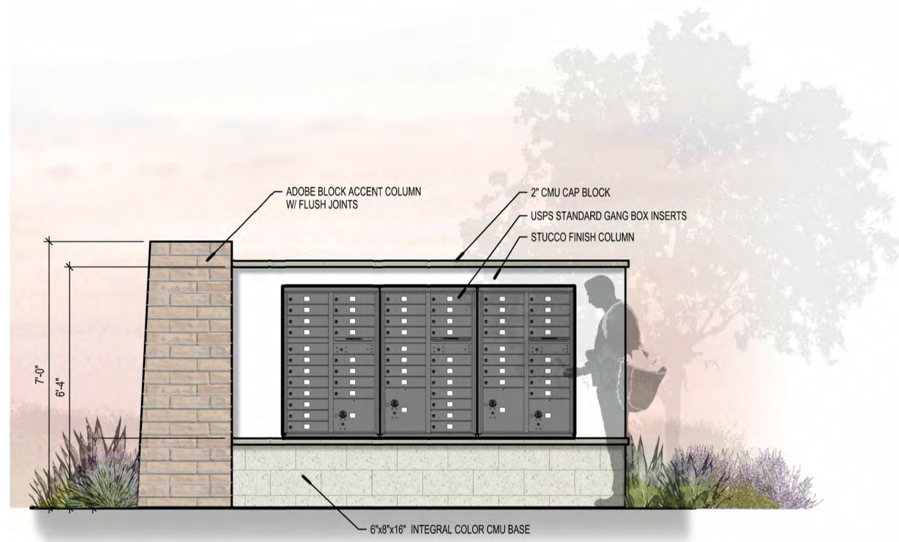
TYPICAL MAILBOX
